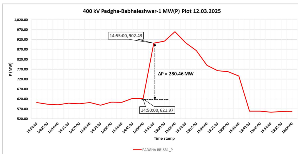
Active Power Flow on 400 kV Babhaleshwar-Padghe-1 (SCADA)
