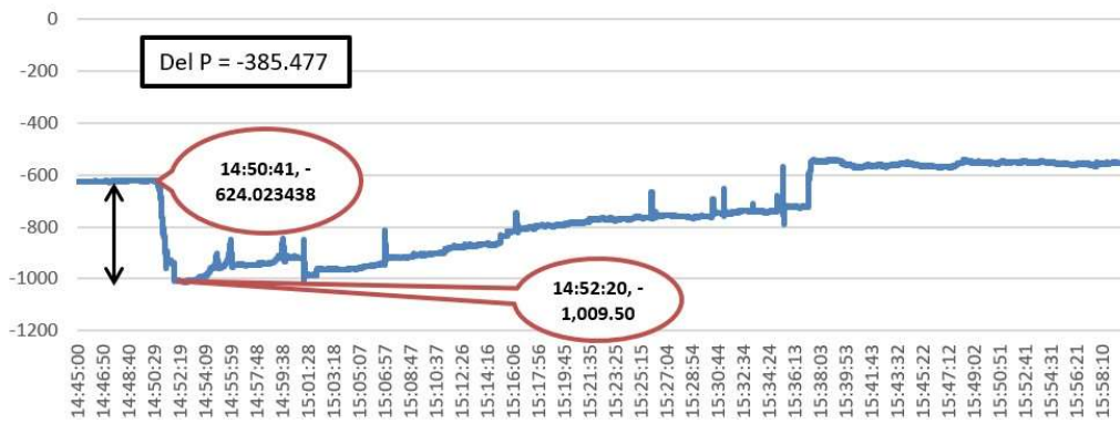
Active Power Flow on 400 kV Babhaleshwar-Padghe-1 (PMU)
