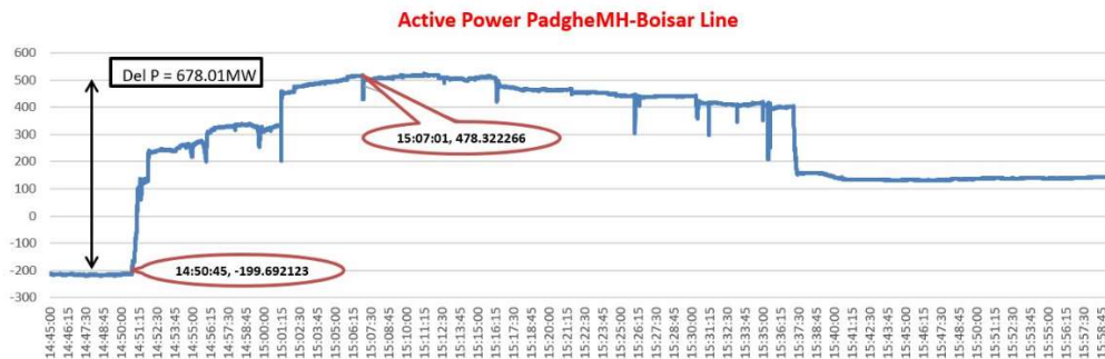
Active Power Flow on 400 kV Tarapur-Boisar (PG) (PMU)
