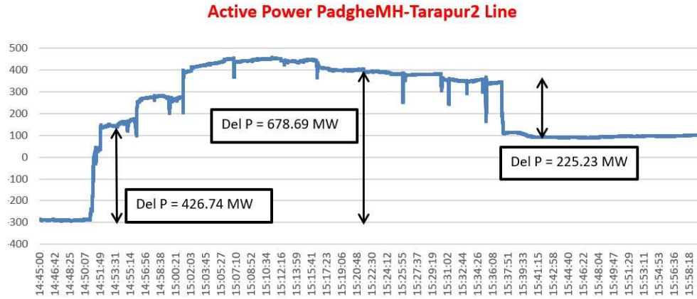
Active Power Flow on 400 kV Tarapur-Padghe-2 (PMU)
