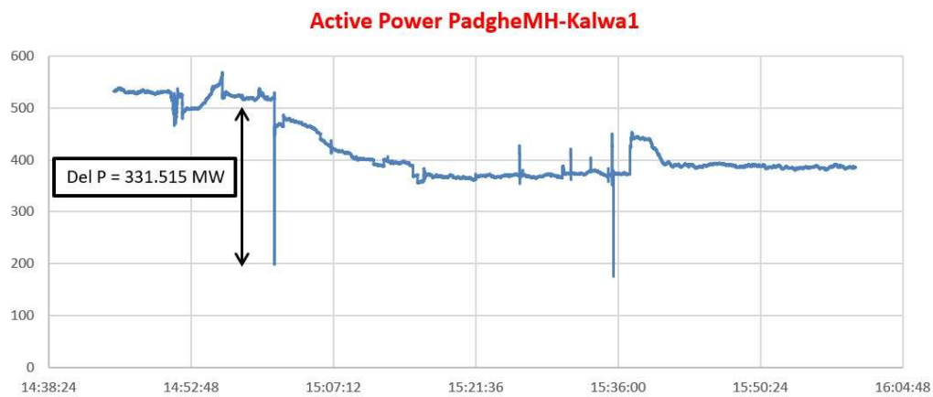
Active Power Flow on 400 kV Padghe-Kalwa-1 (PMU)
