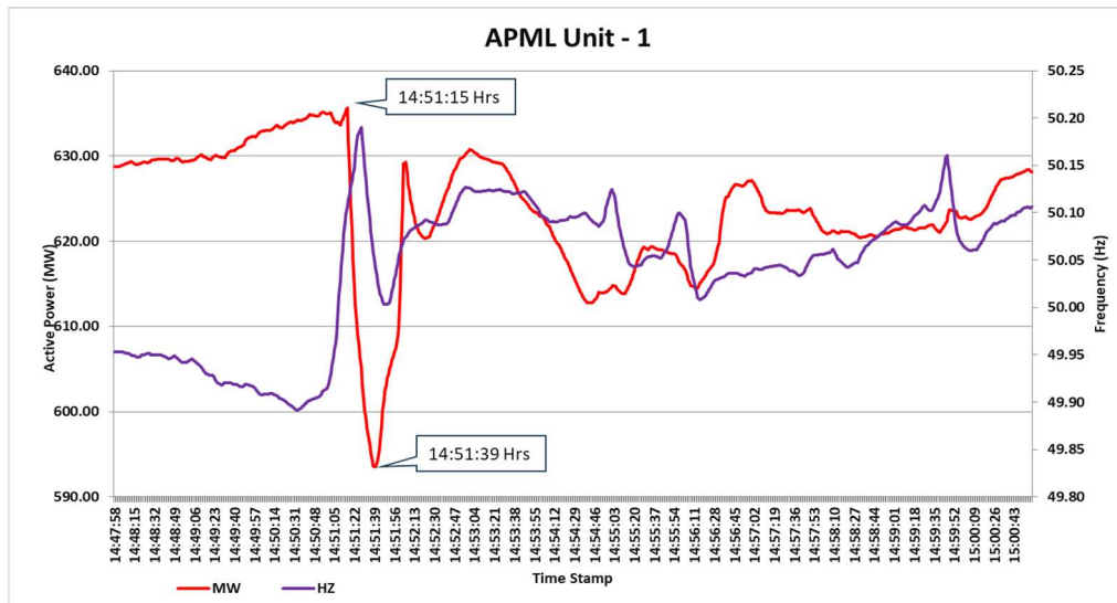
APML Unit-1 (660 MW): Active Power & Frequency (Source: APML)
