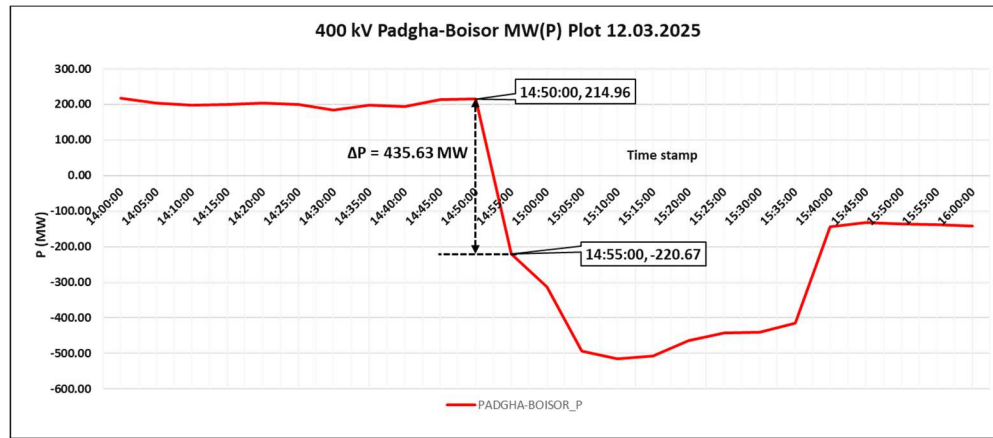
Active Power Flow on 400 kV Tarapur-Boisar (PG) (SCADA)
