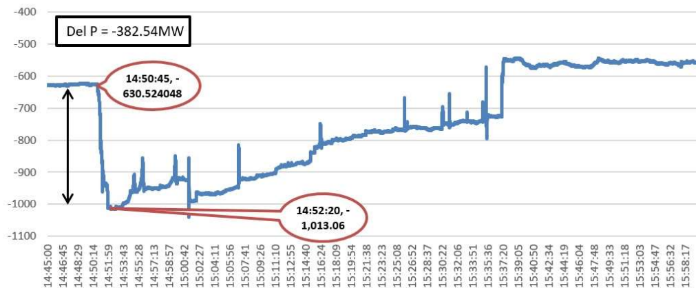
Active Power Flow on 400 kV Babhaleshwar-Padghe-2 (PMU)
