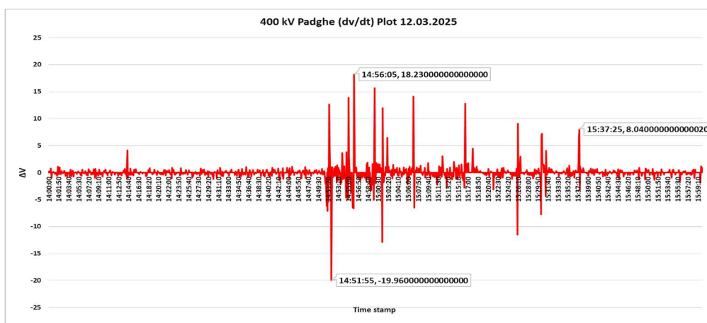
dv/dt plot at 400 kV Padghe S/s. (SCADA)
